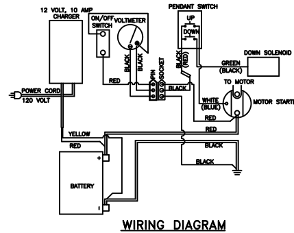
WIRING DIAGRAM
